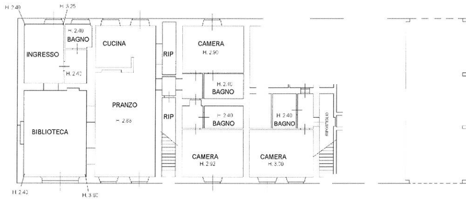
PIANO TERRA
