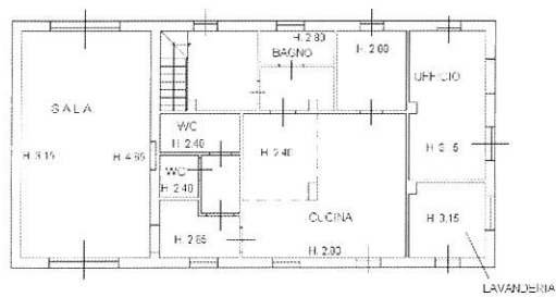
PIANO TERRA
